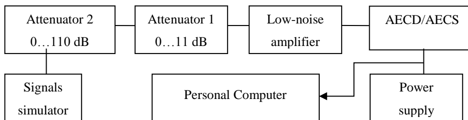
Arrangement for evaluation of GNSS module sensitivity
