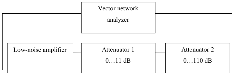
Diagram of path calibration
