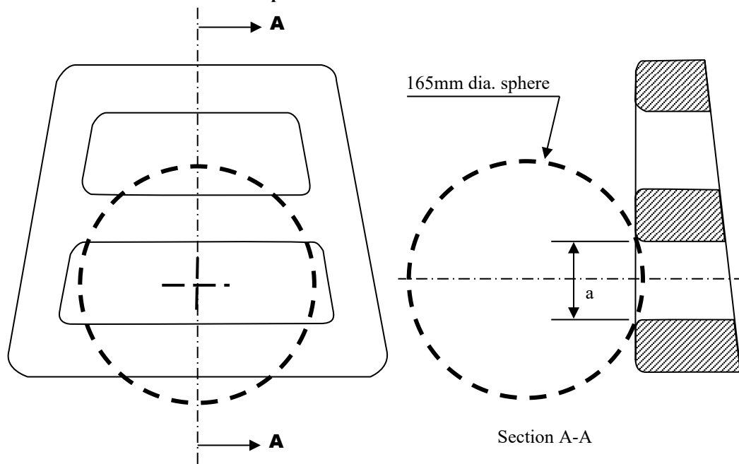
Figure 8-1 Measurement of a Vertical Gap "a"
