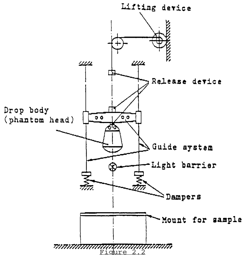
Test apparatus for the headform experiment with deceleration measurement
