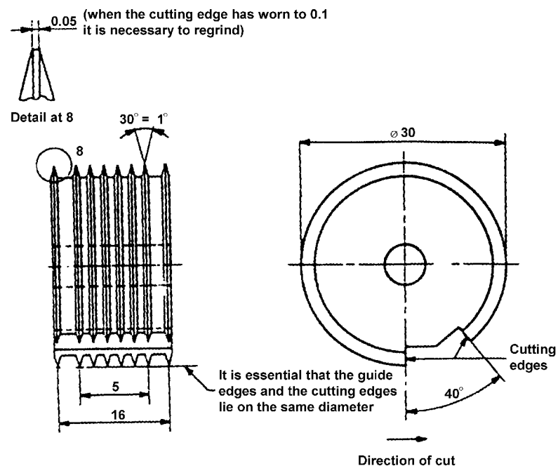
Figure 24: Tool with six blades
