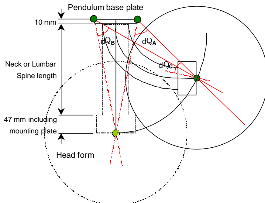
Figure 6 - Neck and lumbar spine certification test set-up (Angles d?A, d?B and d?C measured with head-form)
