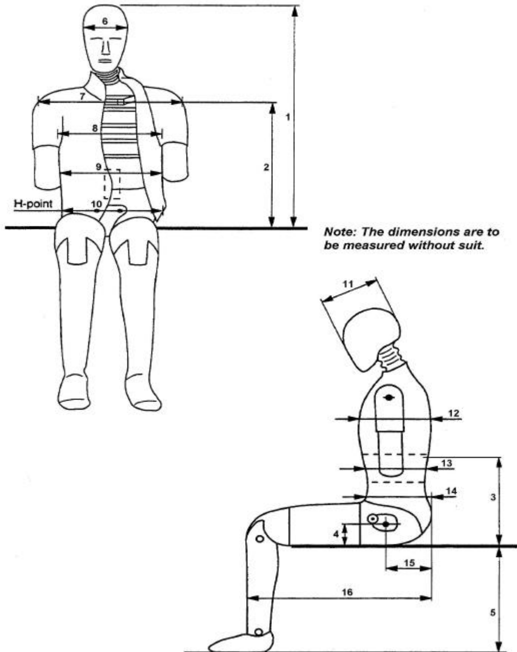
Figure 2 - Measurements for principle dummy dimensions (see Table 3)
