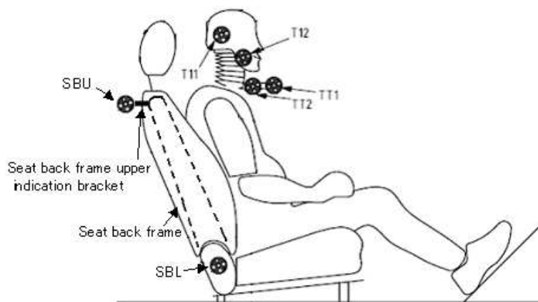
Figure 9-1 Video motion target placements
