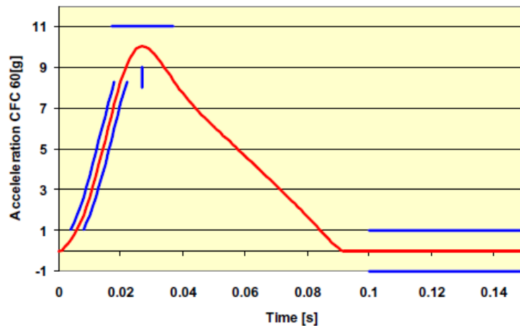
Figure 9-4 Sled pulse
