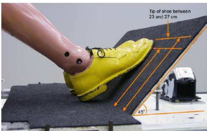
Figure 9-2 Proper positioning of the test dummy's feet.
