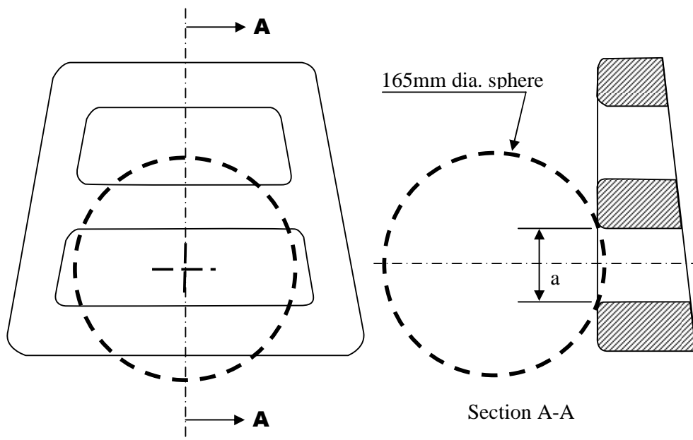
Figure 3-1 - Measurement of a horizontal gap "a".
