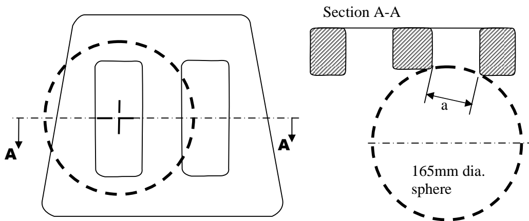
Figure 3-2 - Measurement of a vertical gap "a".
