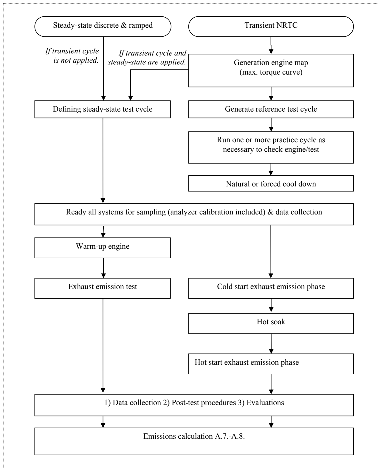
Figure 7.3 Test sequence
