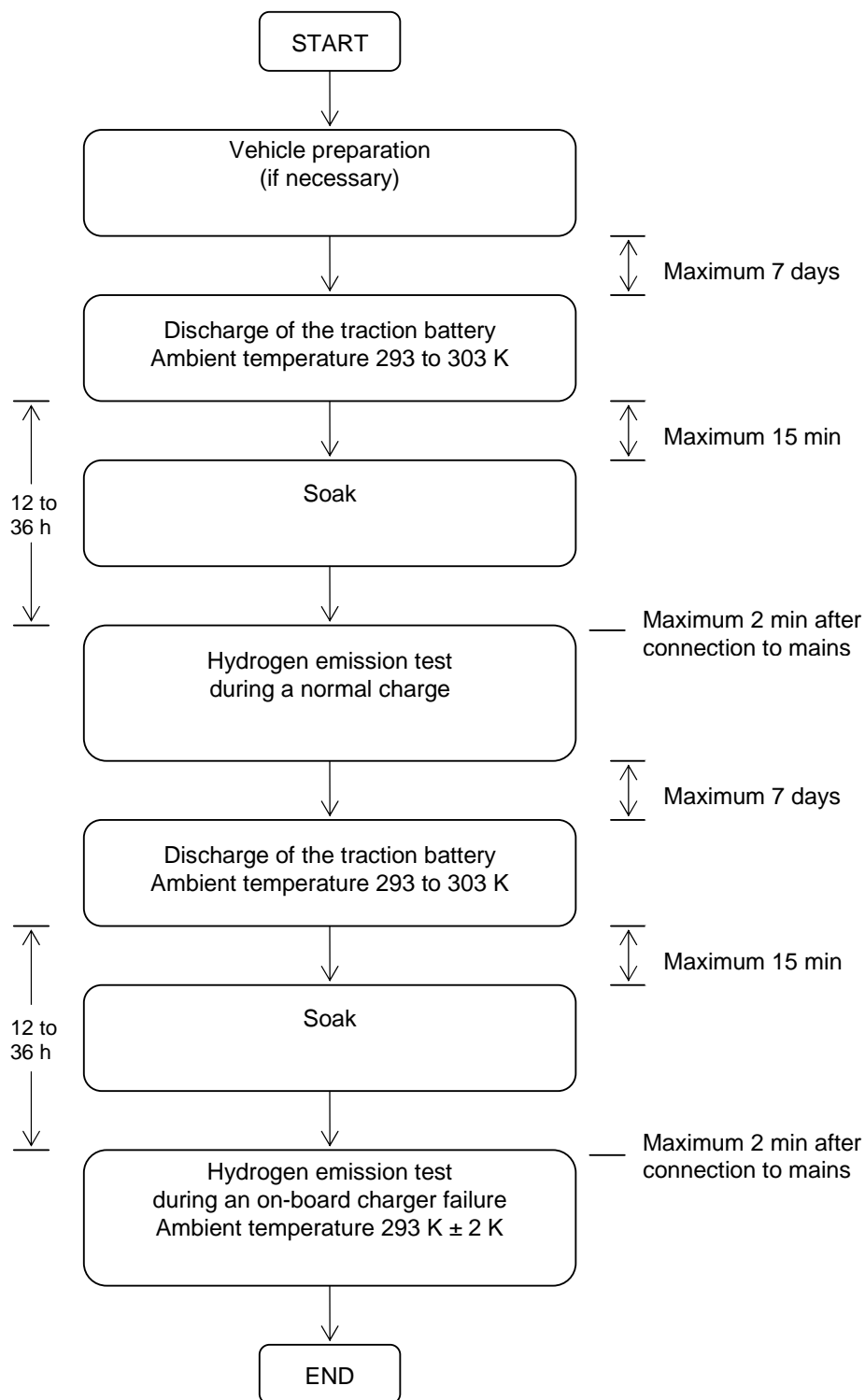
Figure 1 Determination of hydrogen emissions during the charge procedures of the traction battery
